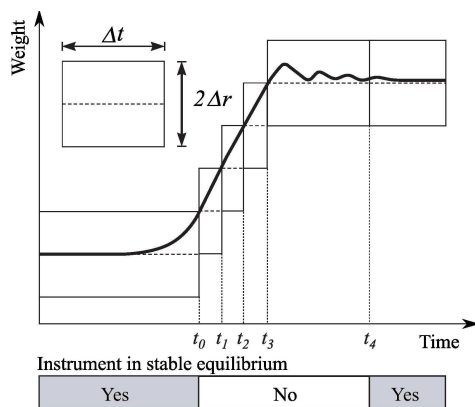
Fig. 2. Criterion for determining the stable equilibrium.
