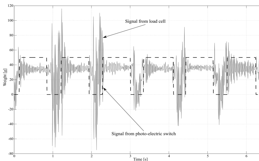
Fig. 3. Time behavior of the catchweigher's measured signals during a weighing process.
