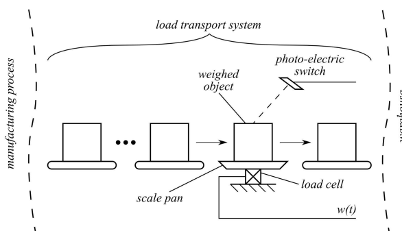
Fig. 1. Static automatic catchweighing instrument.
